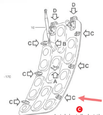
H3198-1UA Latch Assembly
