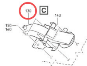
H3198-1UA Latch Assembly
